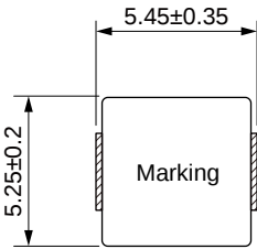
Dimensions: [mm]
