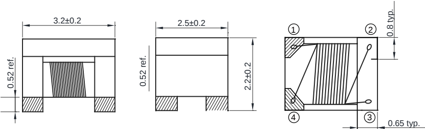
Dimensions: [mm]
